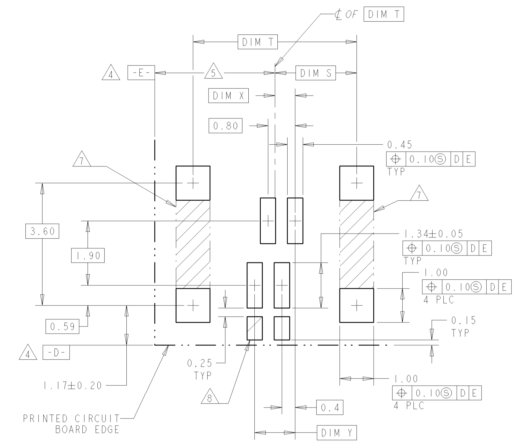
PC BOARD LAYOUT SCALE 15:1
